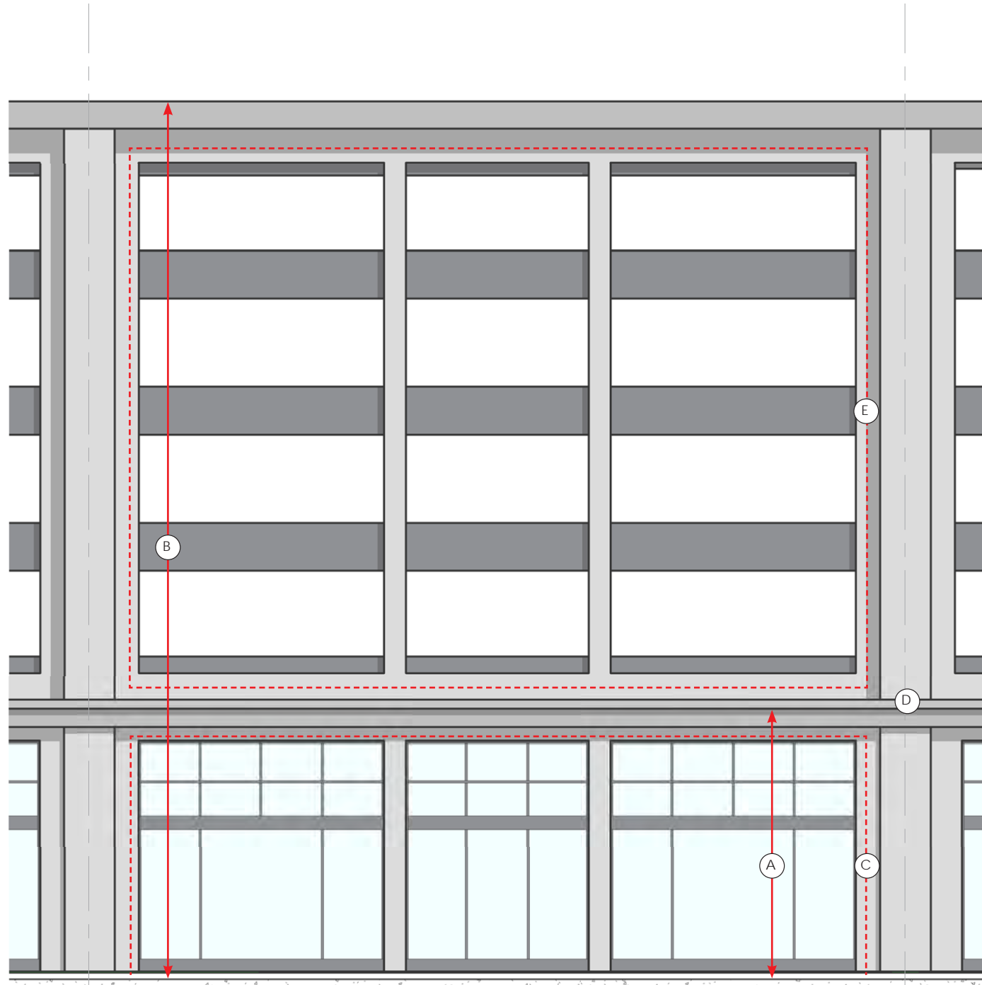
GARAGE DIAGRAM
