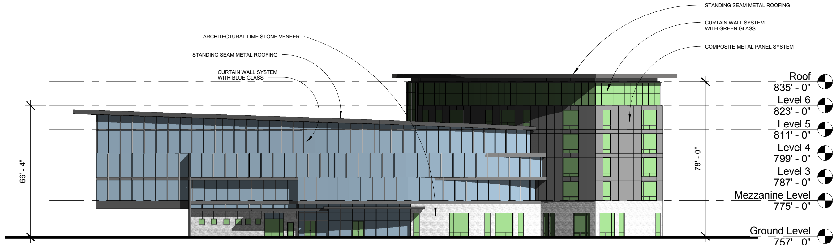
① Old Hickory Blvd Elevation 1" = 30'-0"
