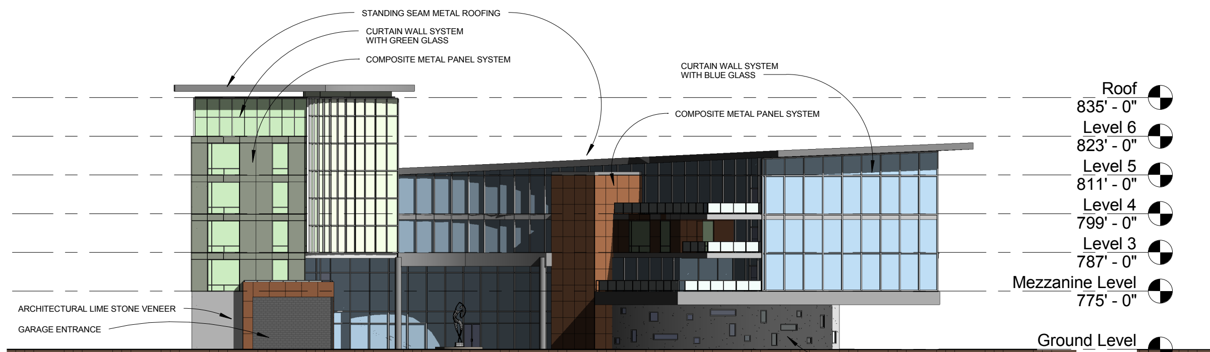
② Franklin Rd. Elevation 1" = 30'-0"
