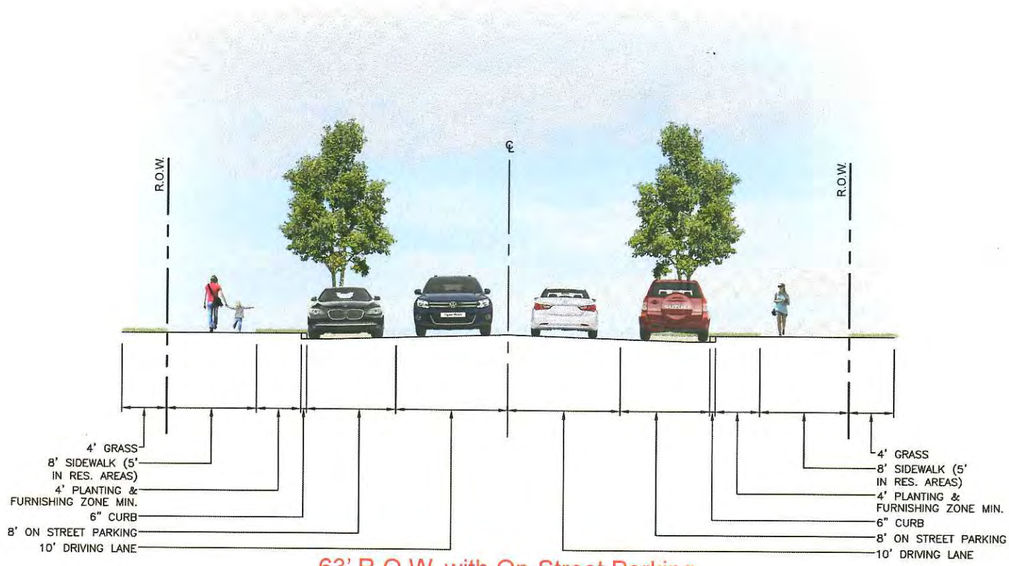
63' R.O.W. with On-Street Parking
