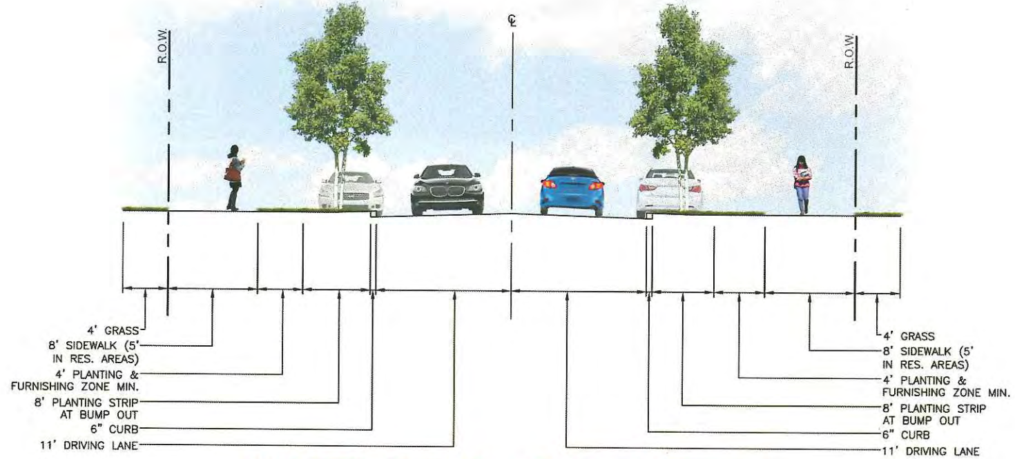
63' R.O.W. with On-Street Parking (At Bumpout)
