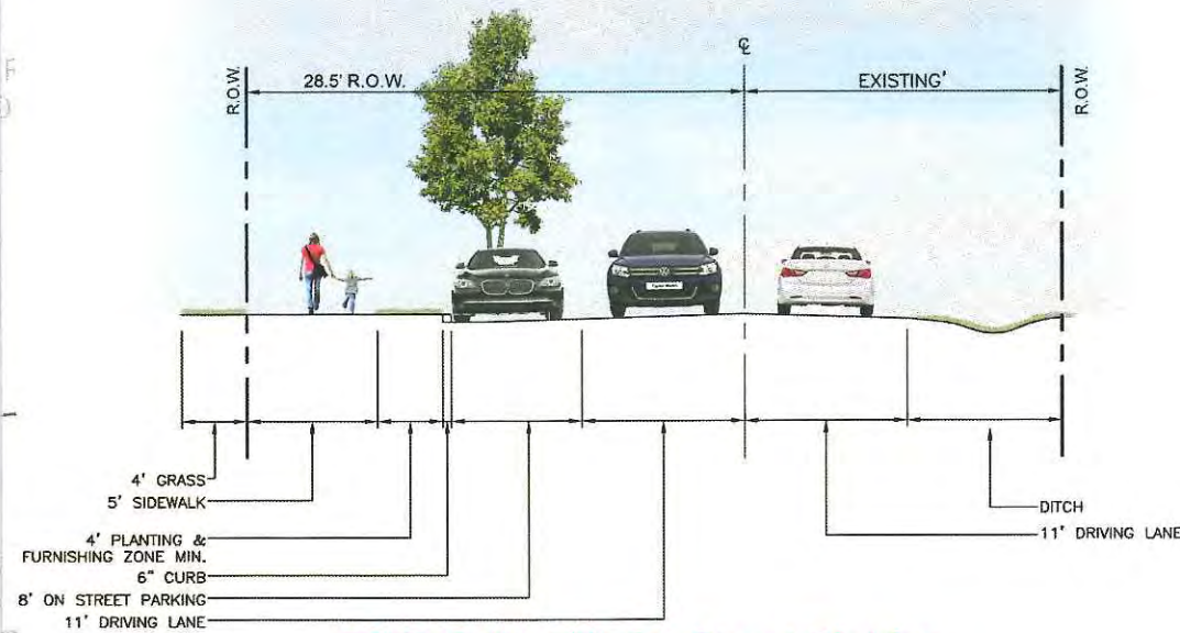
57' R.O.W. with On-Street Parking "Half Section Improvement Only"
