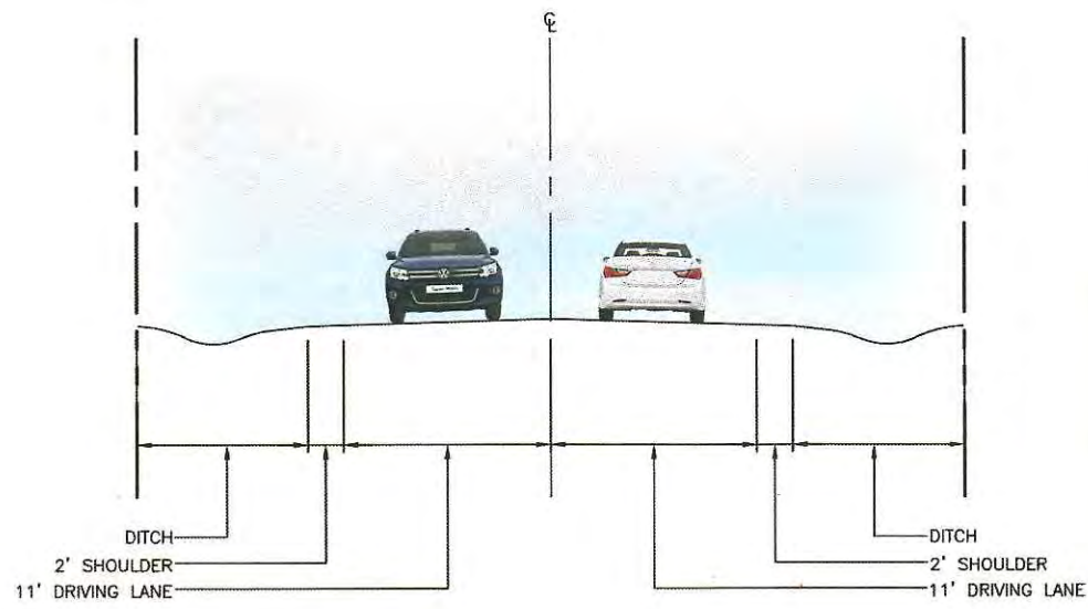
46' R.O.W. with Ditch
